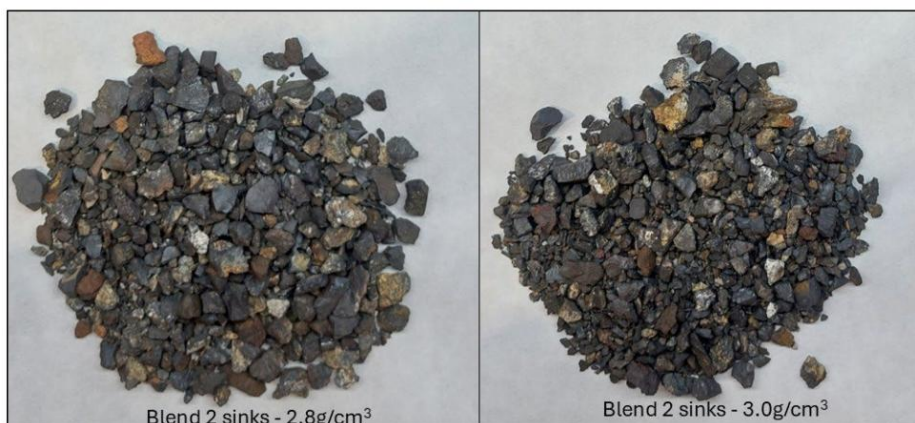
Figure 4. Blend 2 sinks at 2.8g/cm 3 and 3.0g/cm 3 with grades of 41.1% and 43.8% Mn respectively. Pile width is about 15cm.
